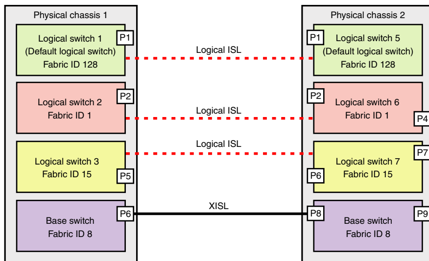
FIGURE 29 Logical ISLs connecting logical switches
